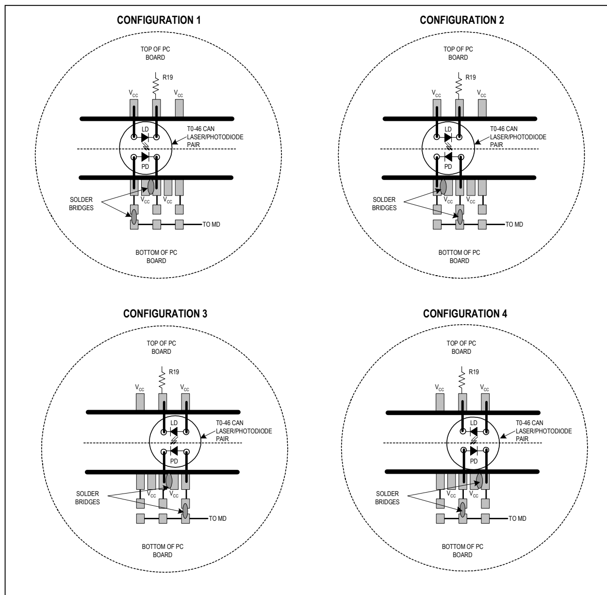
Figure 1. Attachment of Laser Diode/Monitor Diode to the MAX3646 EV Kit
